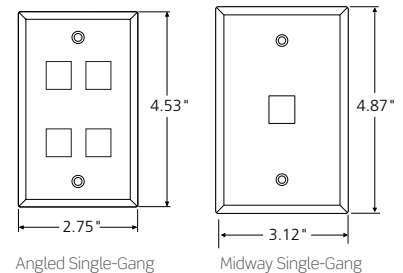
Angled Single-Gang and Single-Gang for Large Connectors
