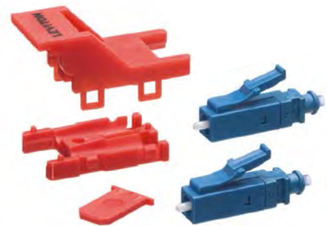
Field-Installable Duplex LC Connector Components
